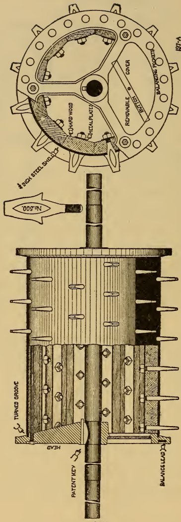
FIG. 67.—“LANDIS ECLIPSE” CLOSED CYLINDER.
